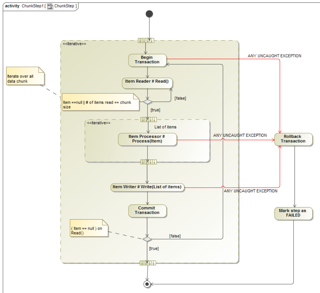
Figure 3.2. Chunk oriented step : when the transaction rollback occurs
