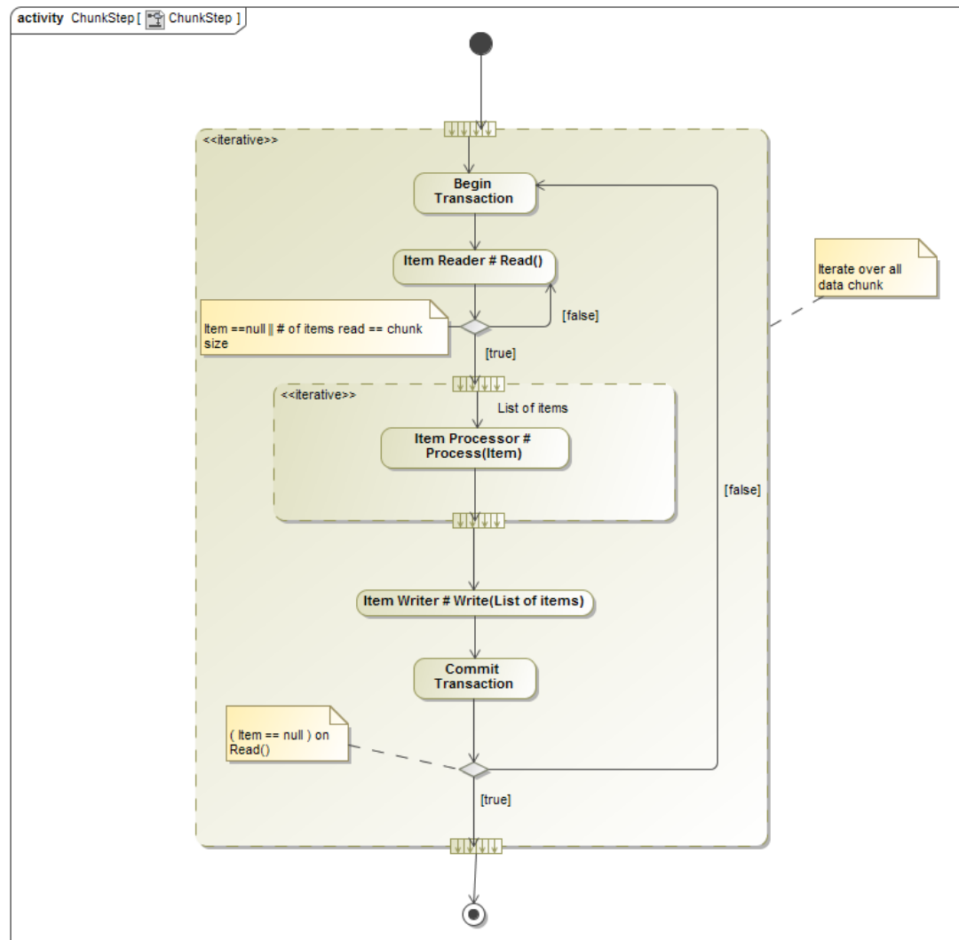
Figure 3.1. Chunk oriented step : basic transactional behaviour
